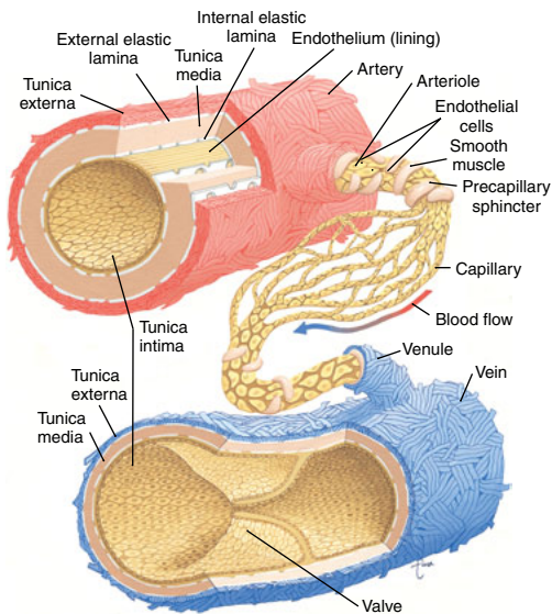
Blood vessels—Cross-section
