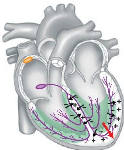
Apical depolarization
