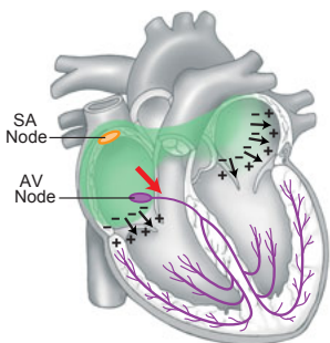
Atrial depolarization
