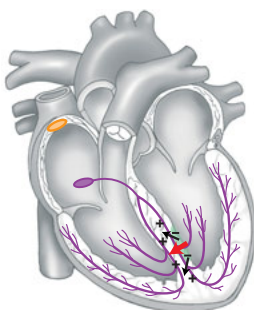
Septal depolarization
